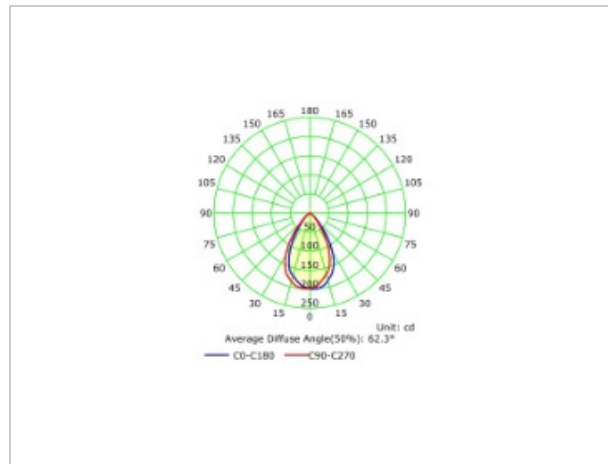
Beam angle / polar diagram
