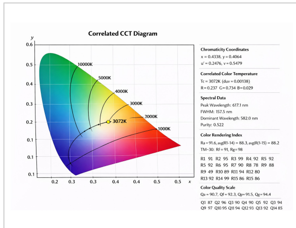
Chromaticity / CCT diagram
